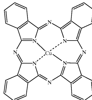
Copper(II) Phthalocyanine(CuPc)
